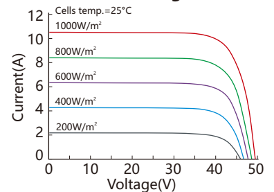
Current-Voltage Curve
