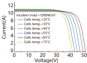
Current-Voltage Curve
