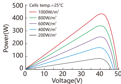
Power-Voltage Curve
